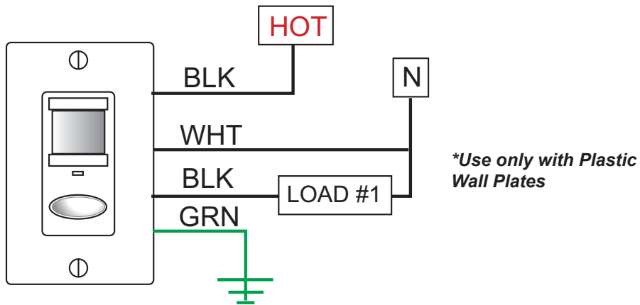
TYPICAL WIRING
